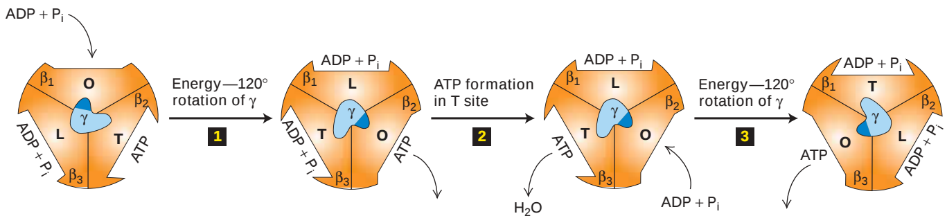
▲ FIGURE 8-26 The binding-change mechanism of ATP synthesis from ADP and P_i by the F_0F_1 complex. This view is looking up at F_1 from the membrane surface (see Figure 8-24). Each of the F_1 \beta subunits alternate between three conformational states that differ in their binding affinities for ATP, ADP, and P_i . Step 1 : After ADP and P_i bind to one of the three \beta subunits (here, arbitrarily designated \beta_1 ) whose nucleotide-binding site is in the O (open) conformation, proton flux powers a 120^\circ rotation of the \gamma subunit (relative to the fixed \beta subunits). This causes an increase in the binding affinity of the \beta_1 subunit for ADP and P_i to L (low), an increase in the binding affinity of the \beta_3 subunit for ADP
