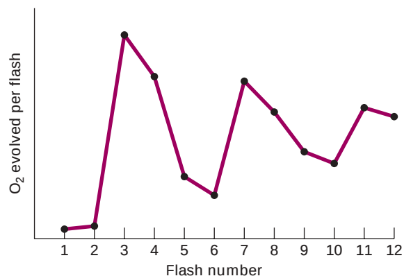
▲ EXPERIMENTAL FIGURE 8-39 A single PSII absorbs a photon and transfers an electron four times to generate one O 2 . Dark-adapted chloroplasts were exposed to a series of closely spaced, short (5-μs) pulses of light that activated virtually all the PSIIs in the preparation. The peaks in O 2 evolution occurred after every fourth pulse, indicating that absorption of four photons by one PSII is required to generate each O 2 molecule. Because the dark-adapted chloroplasts were initially in a partially reduced state, the peaks in O 2 evolution occurred after flashes 3, 7, and 11. [From J. Berg et al., 2002, Biochemistry , 5th ed., W. H. Freeman and Company.]
