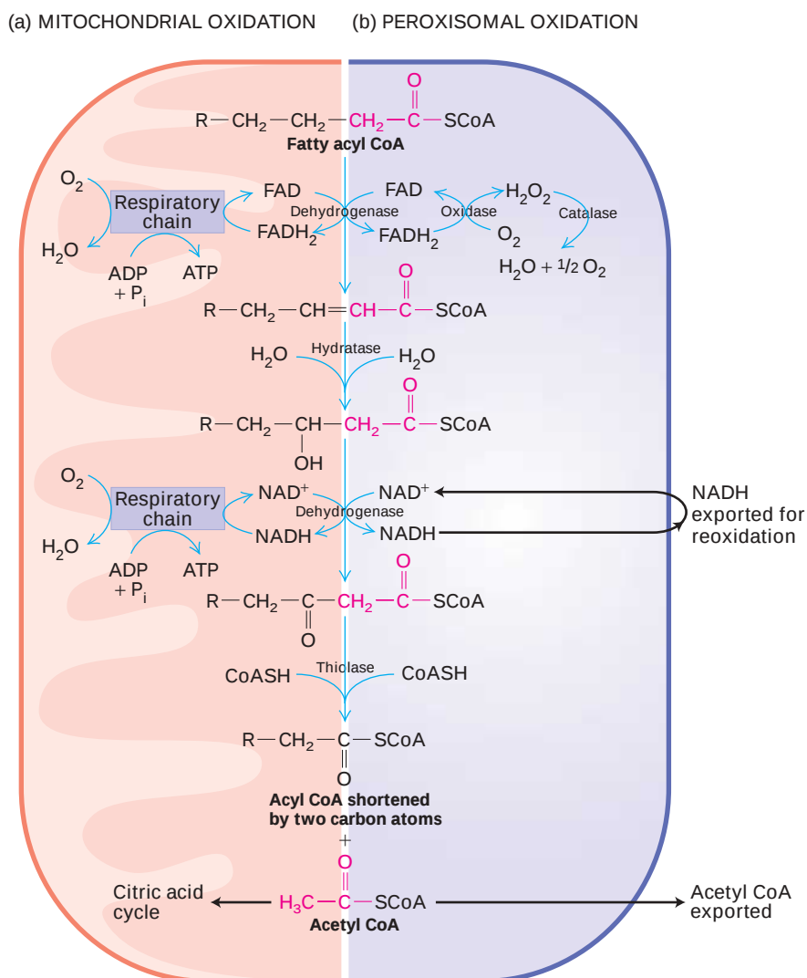
► FIGURE 8-11 Oxidation of fatty acids in mitochondria and peroxisomes.
