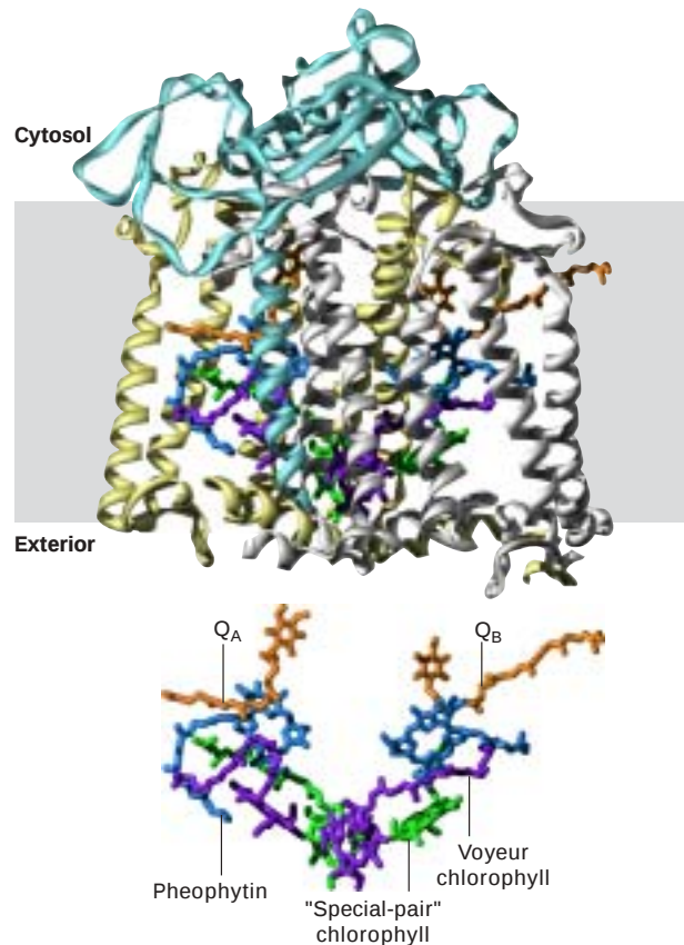
▲ FIGURE 8-35 Three-dimensional structure of the photosynthetic reaction center from the purple bacterium Rhodospirillum rubrum . (Top) The L subunit (yellow) and M subunit (white) each form five transmembrane \alpha helices and have a very similar structure overall; the H subunit (light blue) is anchored to the membrane by a single transmembrane \alpha helix. A fourth subunit (not shown) is a peripheral protein that binds to the exoplasmic segments of the other subunits. (Bottom) Within each reaction center is a special pair of bacteriochlorophyll a molecules (green), capable of initiating photoelectron transport; two bacteriochlorophylls (purple); two pheophytins (dark blue), and two quinones, \text{Q}_\text{A} and \text{Q}_\text{B} (orange). \text{Q}_\text{B} is the primary electron acceptor during photosynthesis. [After M. H. Stowell et al., 1997, Science 276 :812.]
