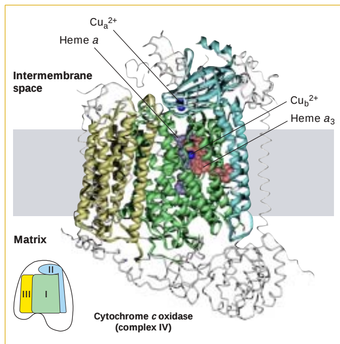
▲ FIGURE 8-18 Molecular structure of the core of the cytochrome c oxidase complex in the inner mitochondrial membrane. Mitochondrial cytochromes c oxidases contain 13 different subunits, but the catalytic core of the enzyme consists of only three subunits: I (green), II (blue), and III (yellow). The function of the remaining subunits (white) is not known. Bacterial cytochrome c oxidases contain only the three catalytic subunits. Hemes a and a 3 are shown as purple and orange space-filling models, respectively; the three copper atoms are dark blue spheres. [Adapted from T. Tsukihara et al., 1996, Science 272 :1136.]
